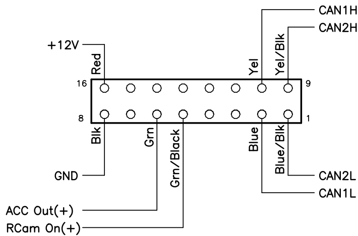
Fig 1 Design and pinout of the module
